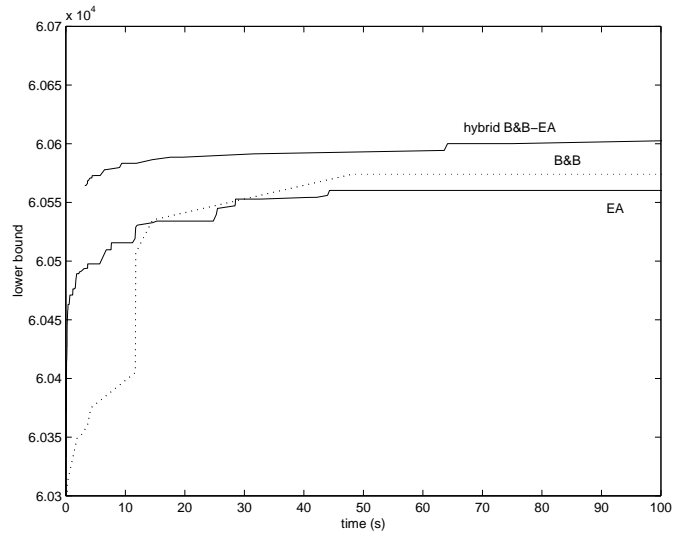
Fig. 3. Evolution of the lower bound in the three algorithms during the first 100 seconds of execution for an problem instance with \alpha = .75 , m = 30 , n = 100 . Curves are averaged for the ten runs in the case of the EA and the hybrid algorithm.
