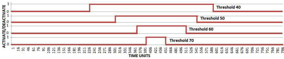
Fig. 10. Activation/Deactivation of support node 1 (n9)
