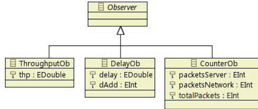
Fig. 7. Observers Metamodel
